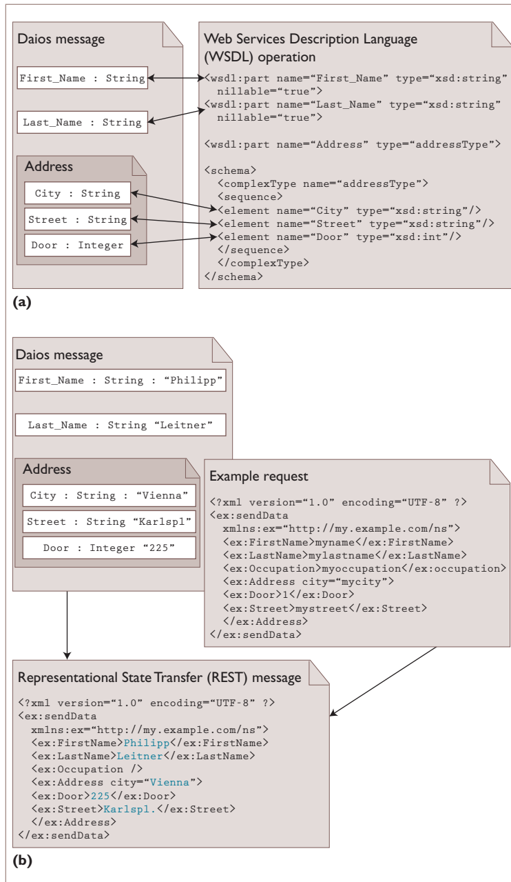
Figure 2. Matching Daios inputs to service interfaces. (a) A Daios message and a WSDL operation with a structural distance of 0. (b) When Daios receives an invocation, it fills the template (example request) with user input to produce a valid REST invocation.
